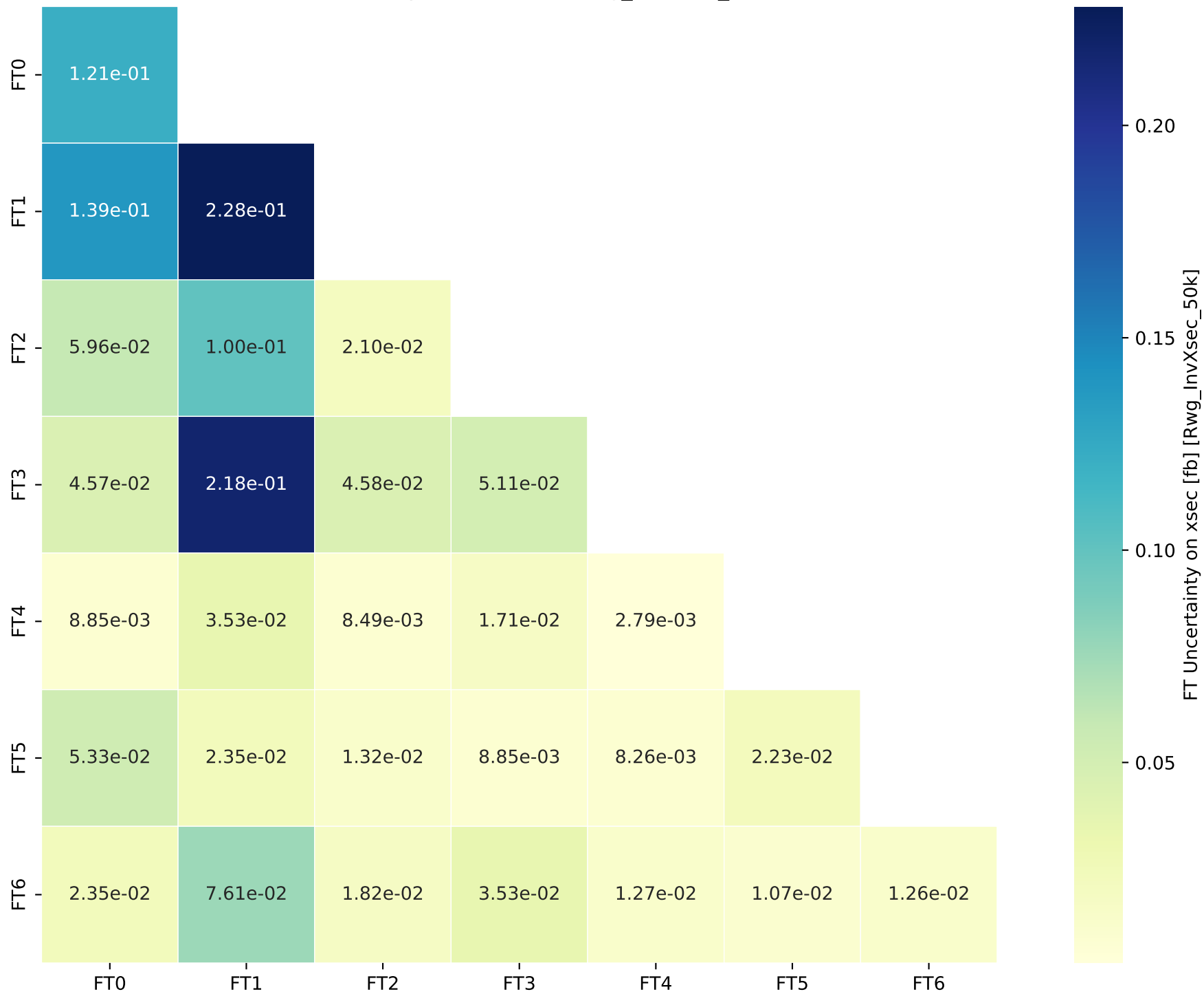
FT Uncertainty on xsec [fb] [Rwg_InvXsec_50k]
